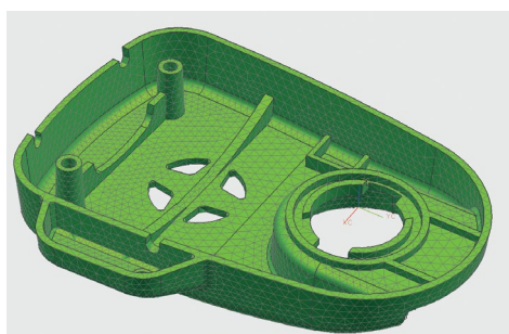
1. Plastic case initial analysis model.
